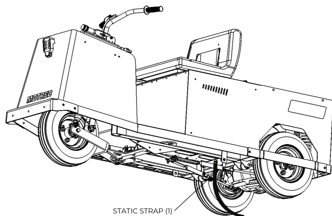
Figure 22. Sangle Anti-statique.
