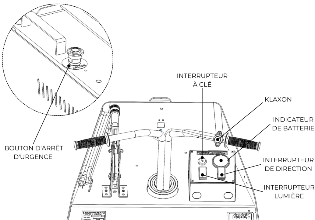
Figure 15. Console.
