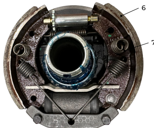
Figure 62. Inspection des sabots et des ressorts.
